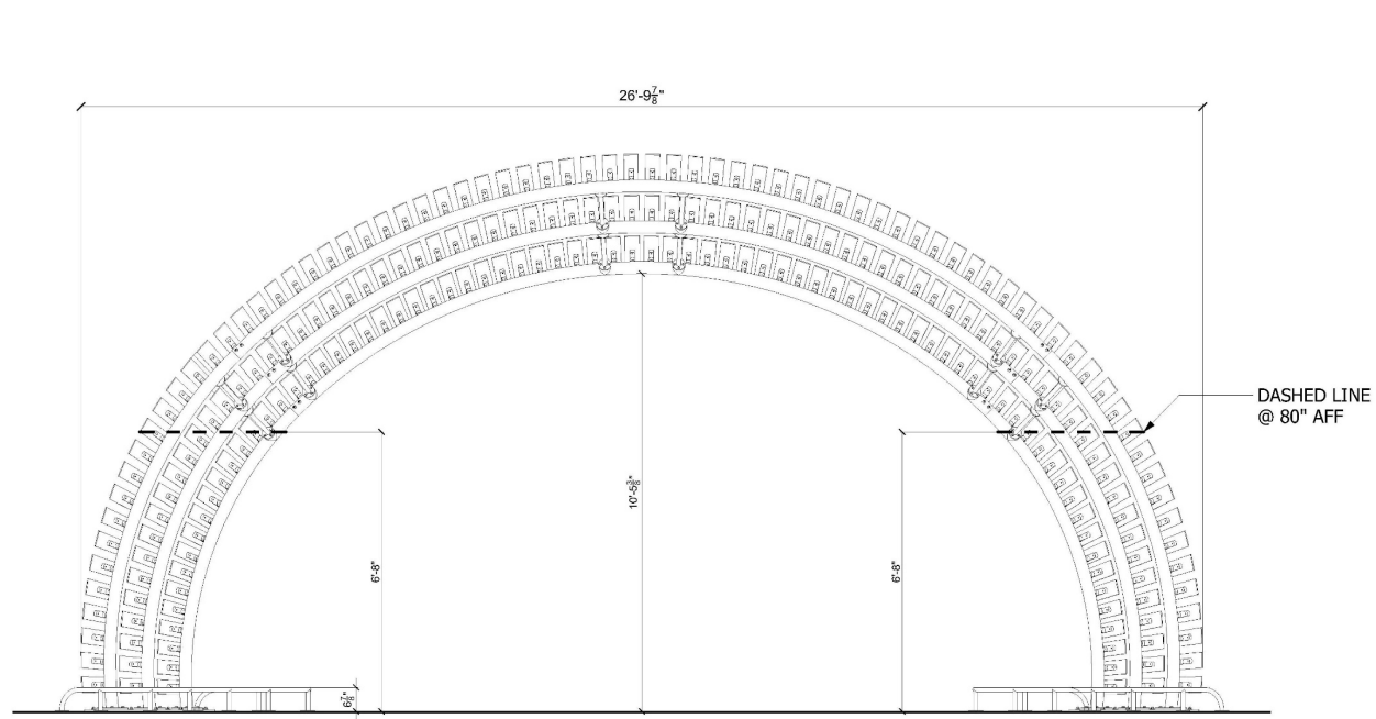
2 FRONT ELEVATION
