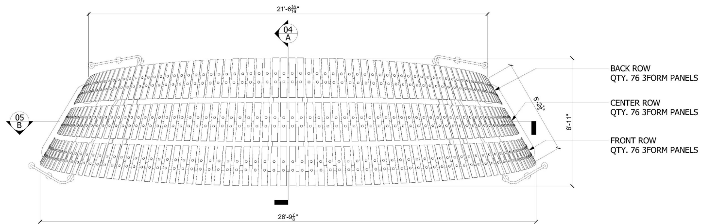
1 PLAN
