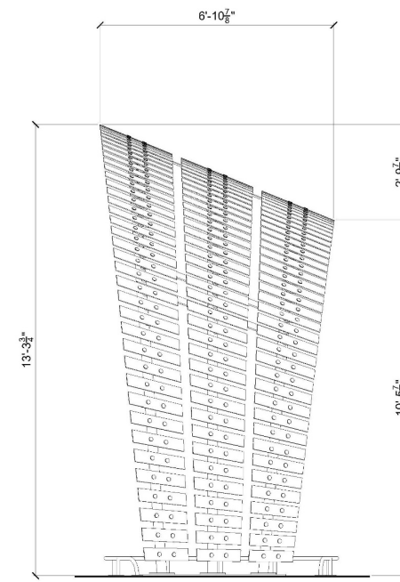
3 SIDE ELEVATION
