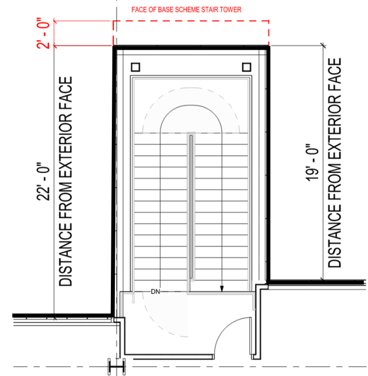
STAIR TOWER – 2'-0" ADJUSTED
