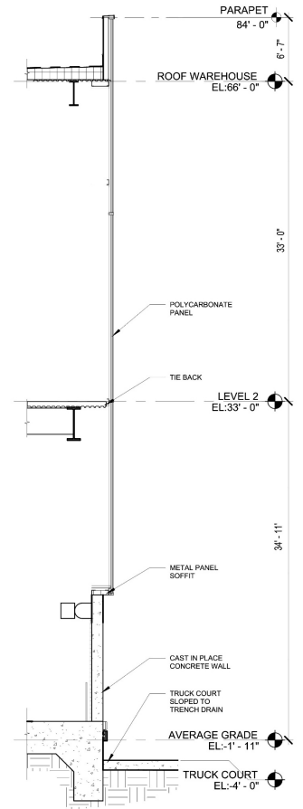
NORTH - WALL SECTION @POLYCARBONATE
